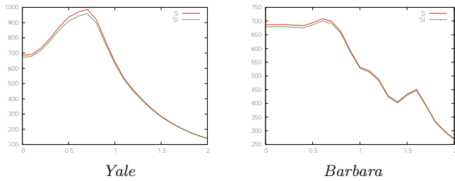
Fig. 8 Blur-ring trade-offs. These diagrams plot the values of SI (in green) and S (in red) of the H^1 regularization u_{\lambda,\rho} defined by (27) with \lambda = 0.01 , as functions of the parameter \rho (in pixels) for images Yale (left) and Barbara (right). SI and S attain their maximum value for a very similar value of \rho , which corresponds in each case to a good trade-off between blur and ringing for these images (see Fig. 9).
